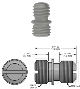
MH108-5B 1/4-28 to M6x1 adapter stud stainless steel
