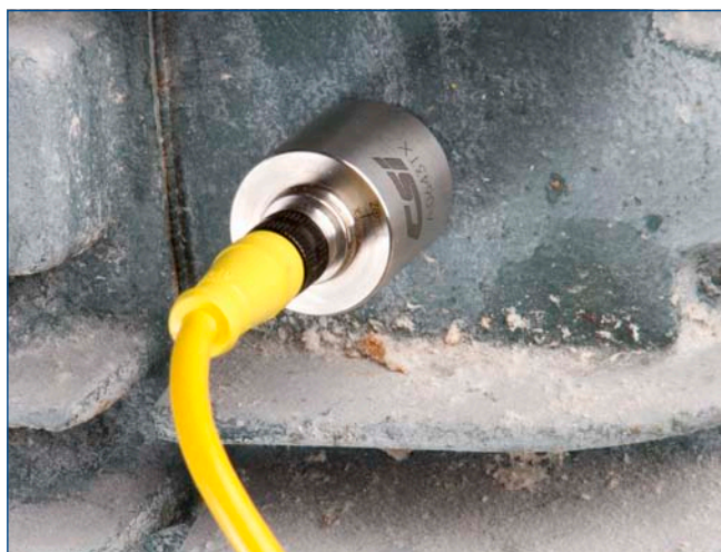
The triaxial accelerometer collects data at the measurement location from a vertical, horizontal, and axial directions simultaneously.
