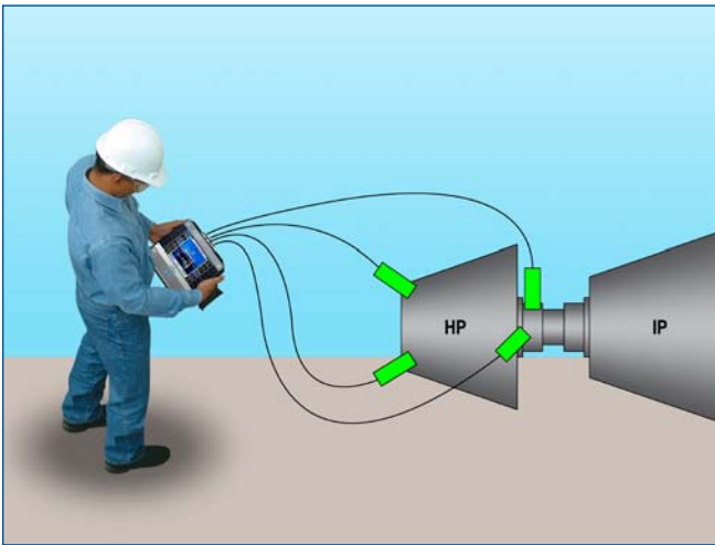
The CSI 2140 provides four-channels of simultaneous data collection plus phase, delivering real-time views into the most complex machinery problems.
